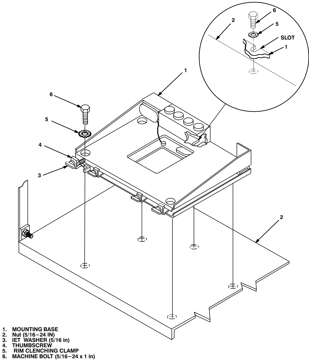
Figure 5-5. Mounting Base Installation: Roadside
