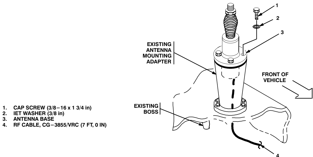
Figure 5-2. Antenna Base Installation: Front Roadside
