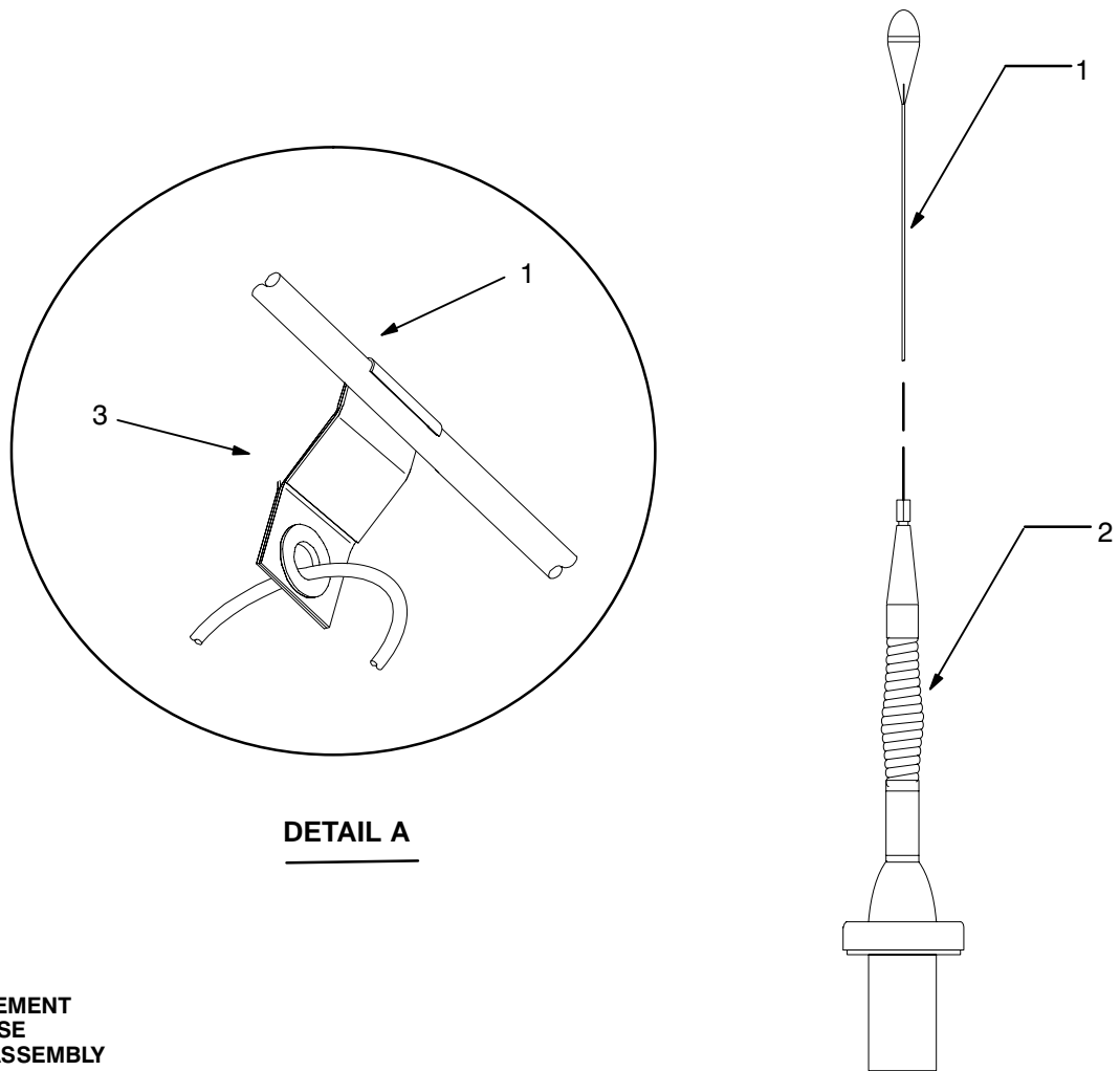
Figure 5-3. Top Antenna Assembly Installation
