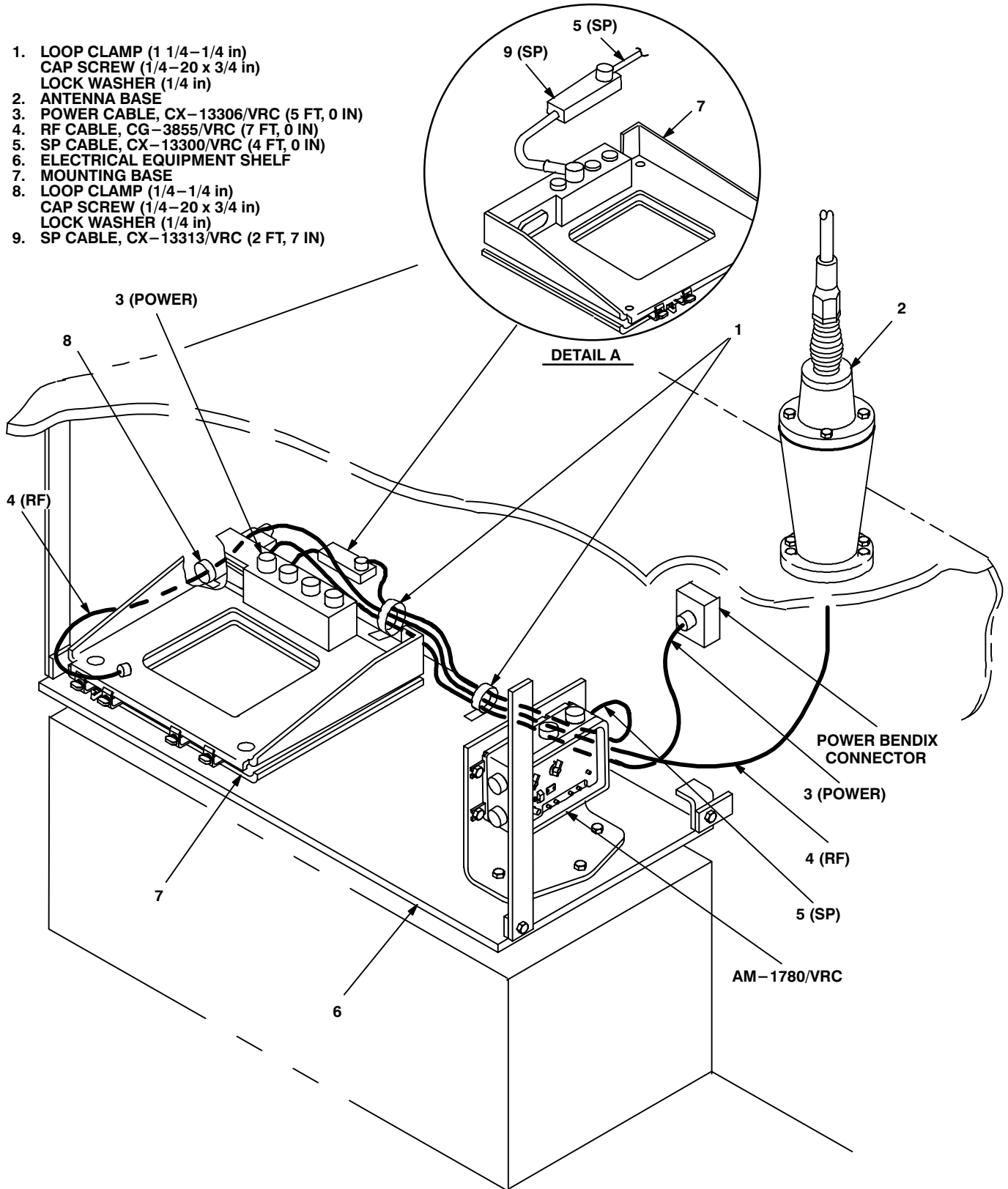
Figure 5-6. Cable Installation: Roadside Interior
